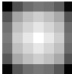
Recovered PSF
