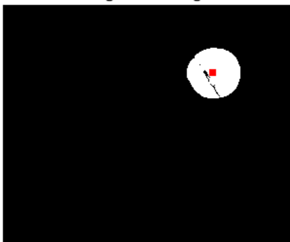
Segmented Image
