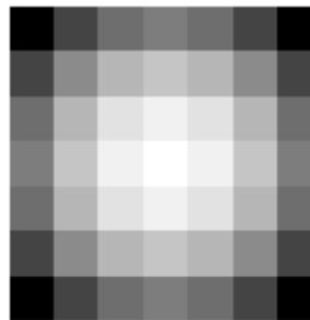
True PSF
