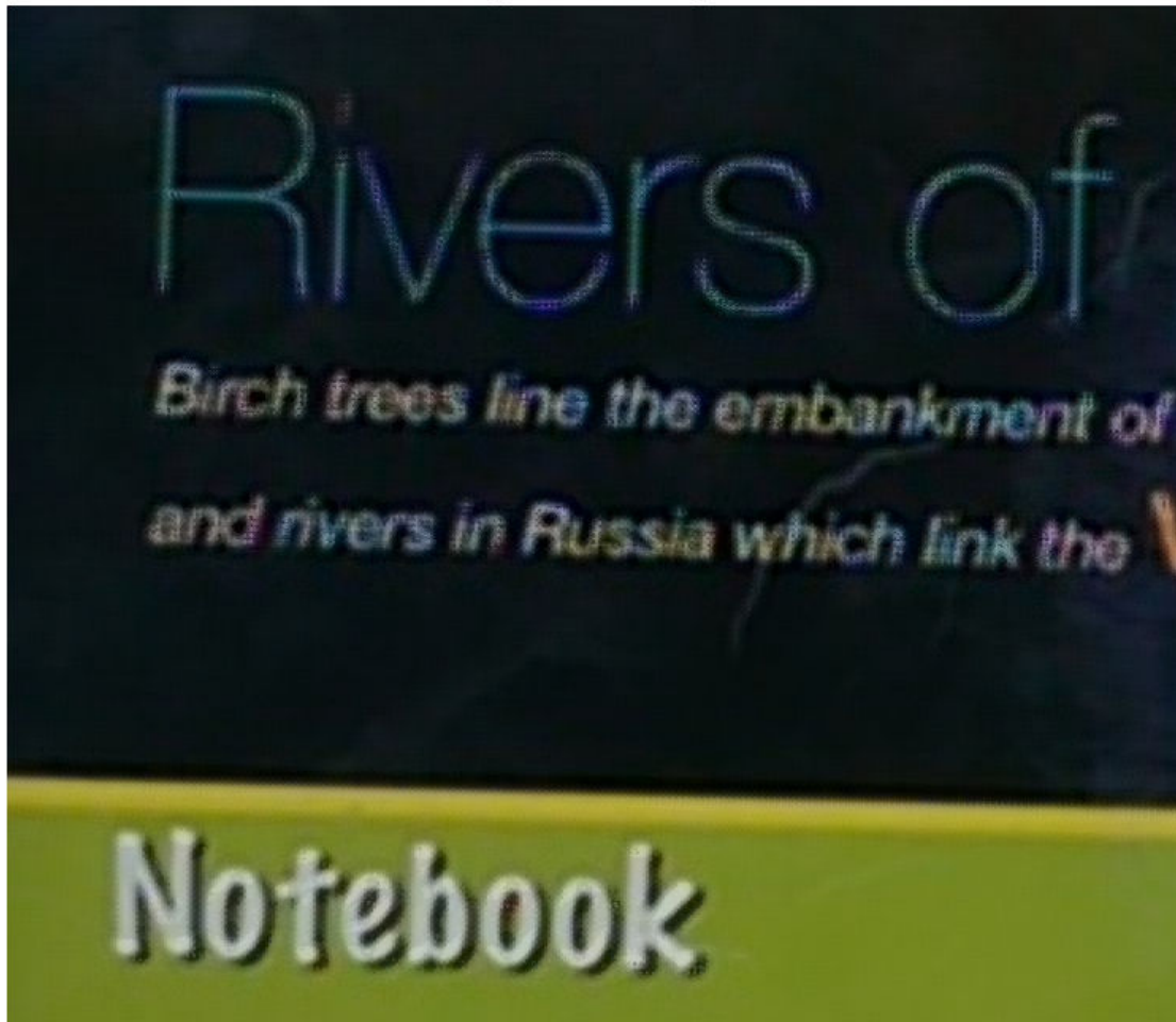
High-Resolution Image
